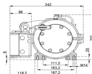
Manual Clutch
