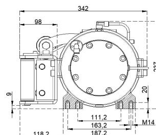
Air Clutch
